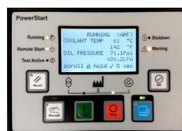
PowerStart 600 control operator/Display
